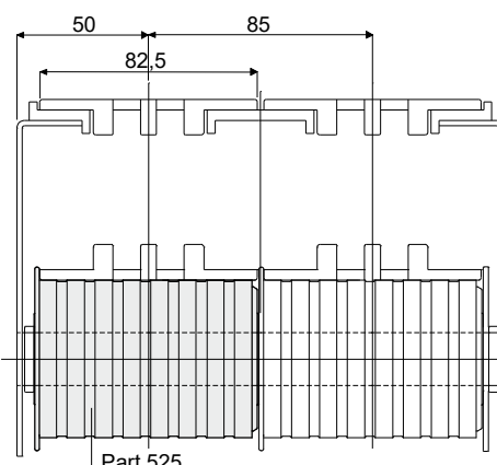
Part.525
