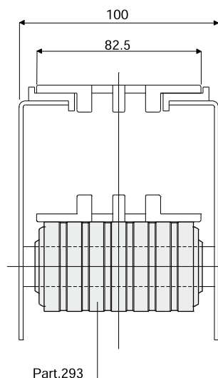
Part.293
